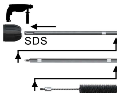
Wire brush R-BRUSH-TC, extension with SDS tit R-BRUSH-EXT-H-SDS, extension R-BRUSH-EXT-H-TC for automatic cleaning
