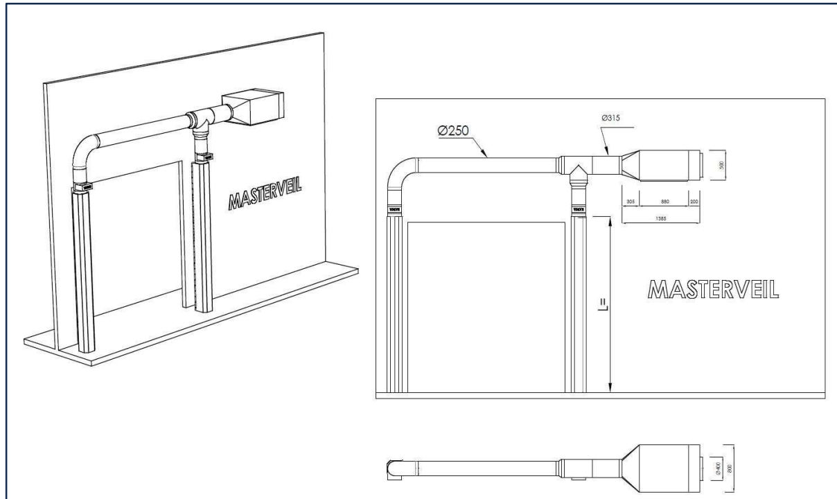
AS 40K double standing air curtains, connection box.
