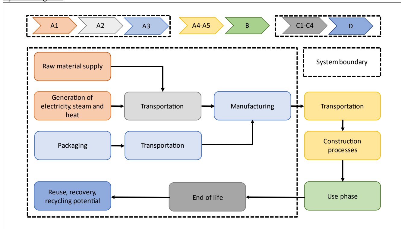
Figure 1 System boundary of the LCA study conducted on Fatra homogeneous waterproofing membranes
